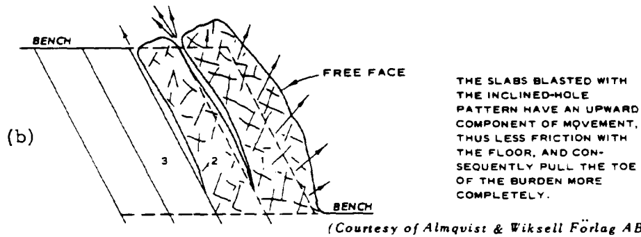
Fig. 5-7. Bench-slab movement during blast with vertical (a) and inclined (b) holes (after Langefors and Kihlström 14 )
