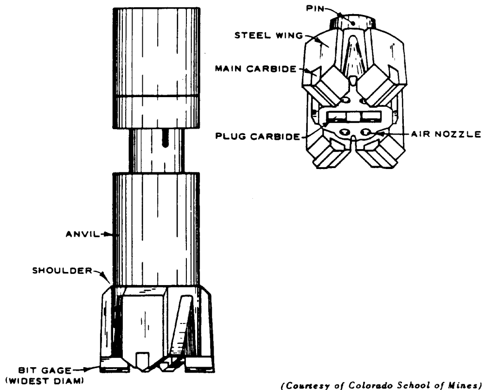
Fig. 4-14. Rotary-percussive drill bit (after Liljestrands 13 )
