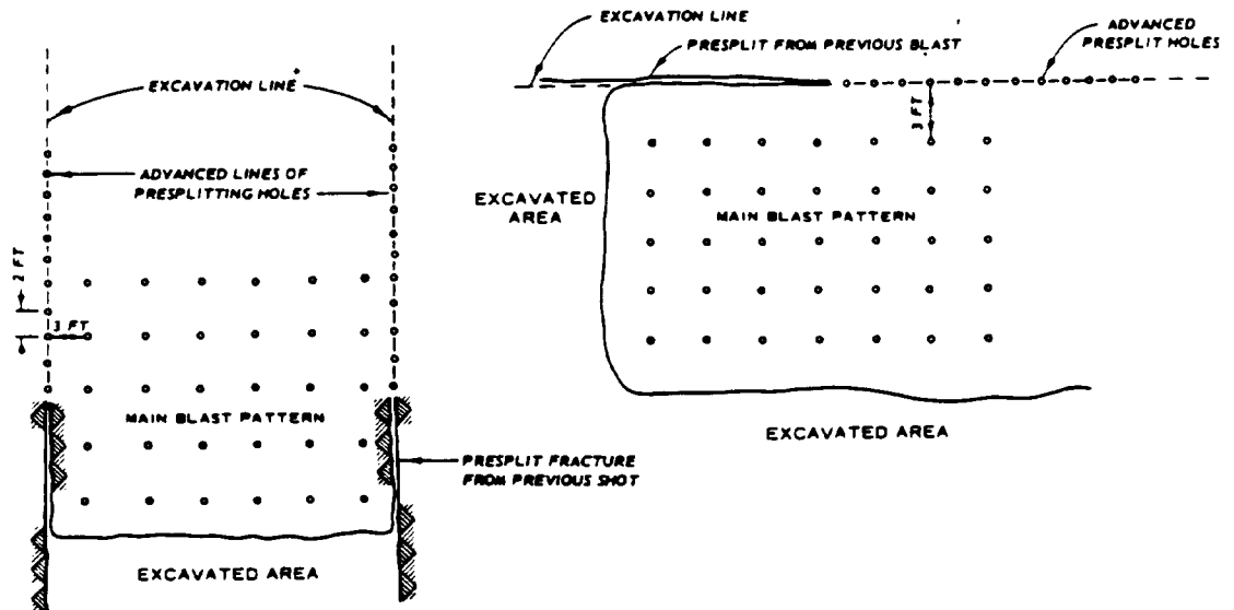
b. PLAN OF TYPICAL SIDE-CUT OR BENCH BLASTING PATTERN
